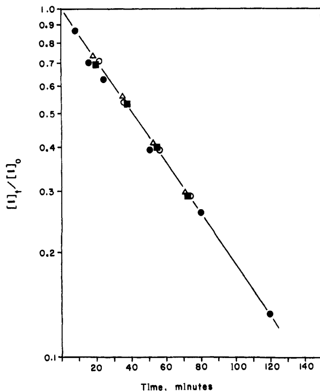
Figure 8. Thermal decomposition of 1 at 69 °C in benzene (●) and in 0.04 M (■), 0.08 M (○), and 0.16 M (Δ) solutions of bis(dicyclohexylphosphino)ethane in benzene. [I]_0 = 0.08 M.
