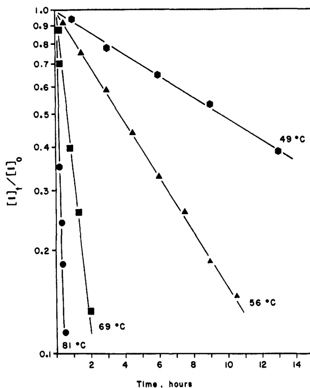
Figure 2. Thermal decomposition of 1 in benzene. [\text{I}]_0 = 0.08 M.
