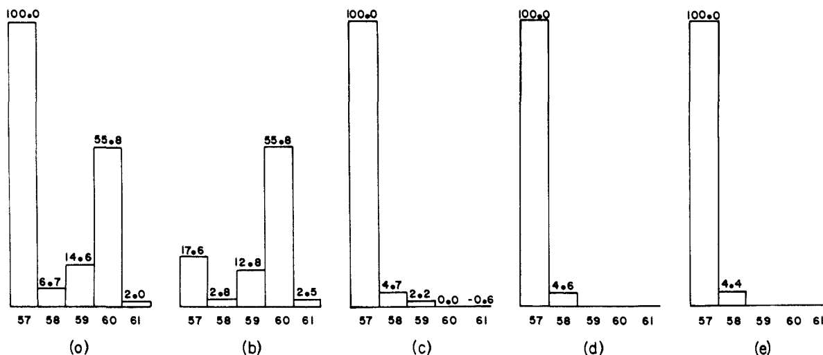
Figure 14. GC/MS analysis of neopentane: (a) neopentane from the thermal decomposition of equimolar amounts of 1 and 6-d 3 in C 6 H 6 at 69 °C; (b) neopentane from the thermolysis of 6-d 3 in C 6 H 6 at 69 °C, normalized such that the intensity of the base peak, m/e 60, is 55.8%; (c) spectrum a - spectrum b, normalized so that the intensity of the base peak, m/e 57, is 100%; (d) mass spectrum of authentic neopentane; (e) MS of the neopentane produced by thermal decomposition of 1 in C 6 D 6 .
