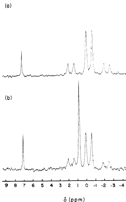
Figure 11. 2 H NMR spectra of 1-d 1 in C 6 H 6 at t = 0 (a) and t = 65 min at 69 °C (b). The doublet at \delta -0.20 corresponds to the deuterium ligand bonded directly to the platinum center; the singlet at \delta 0.87 corresponds to neopentane- d 1 . No peaks are observed at \delta 2.53 (PtCHDCMe 3 ) or \delta 1.70 (PtCH 2 C(CH 3 ) 2 (CH 2 D)).
